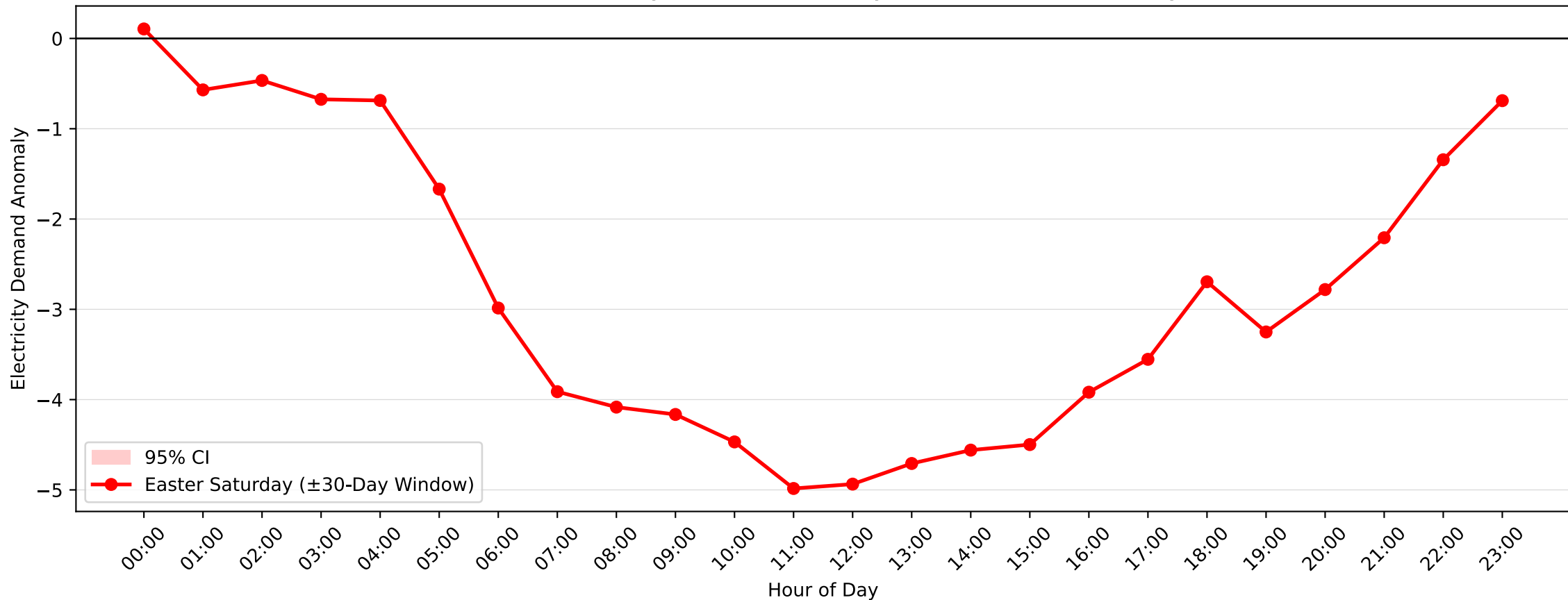
Sefton Demand Anomaly: Easter Saturday (2017-2018, \pm 30 -Day Window)
